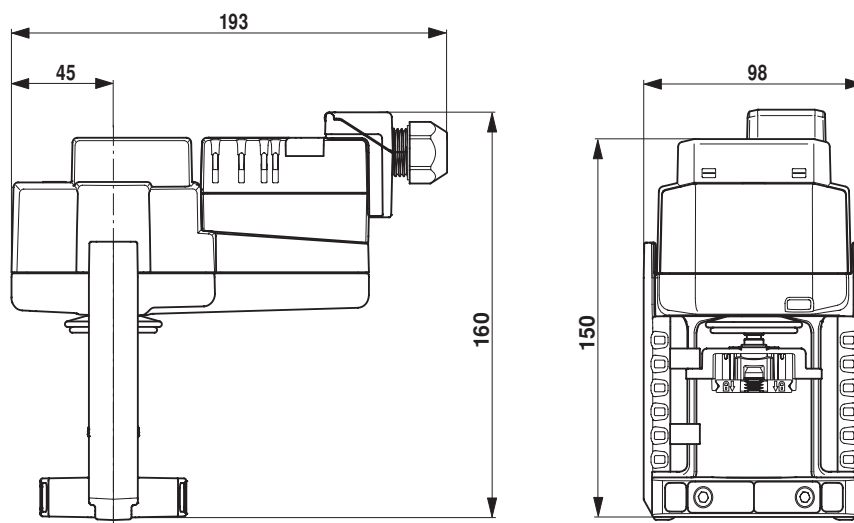
Dimensional drawings
